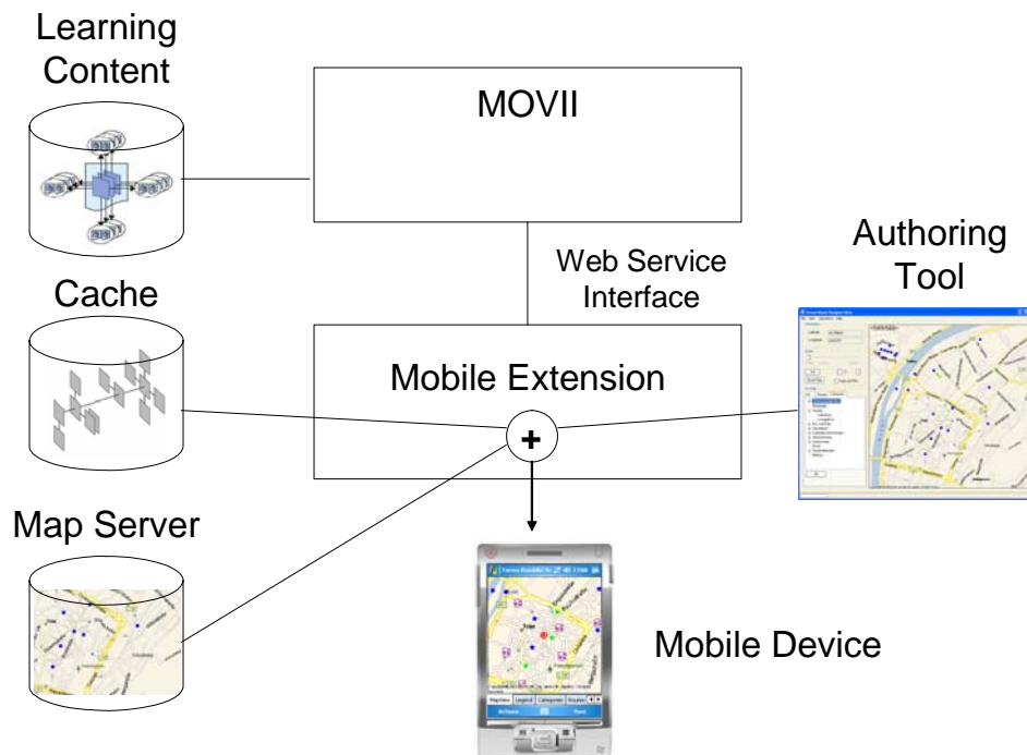
Figure 2: System Architecture.
